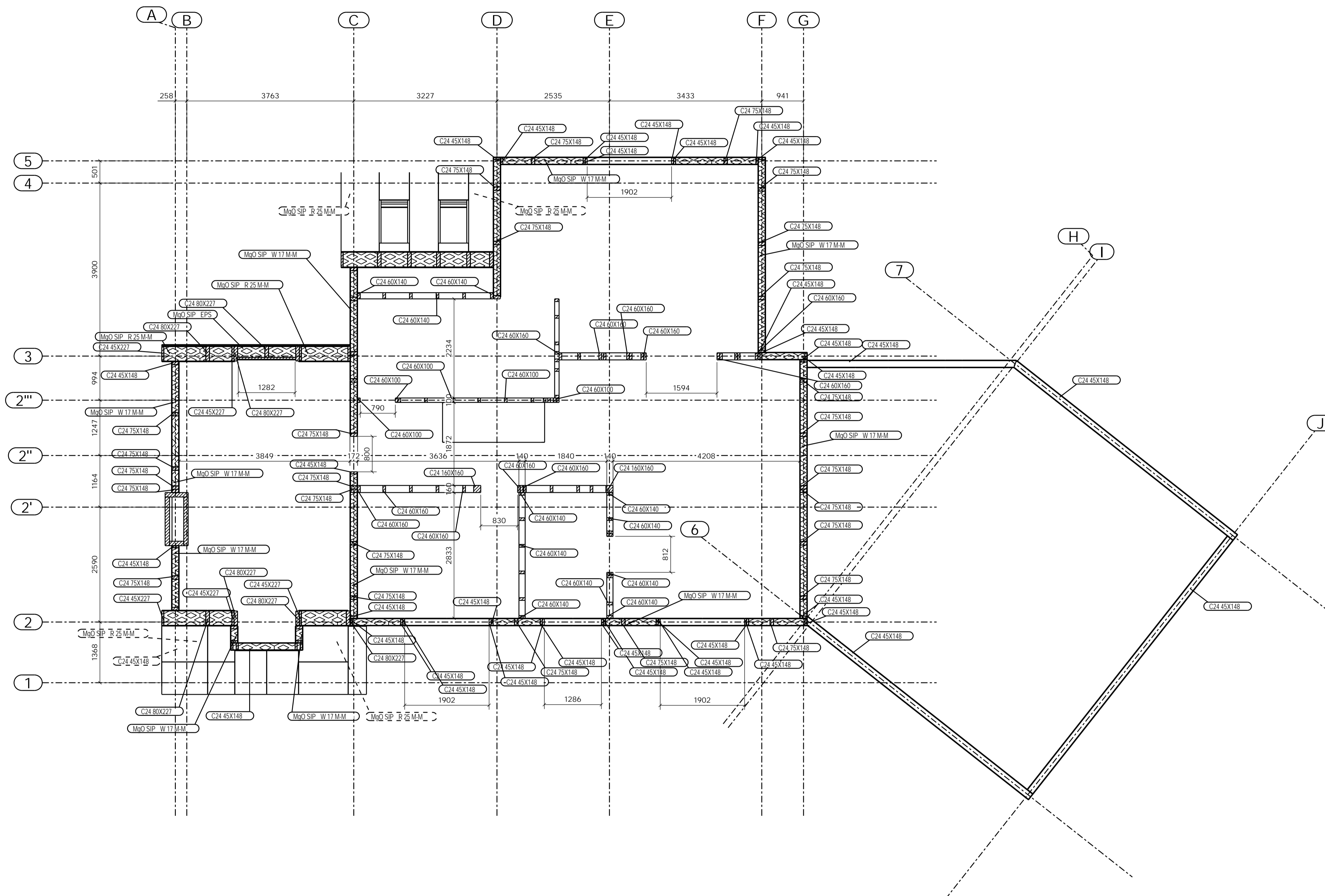
FIRST FLOOR PLAN 1:50
