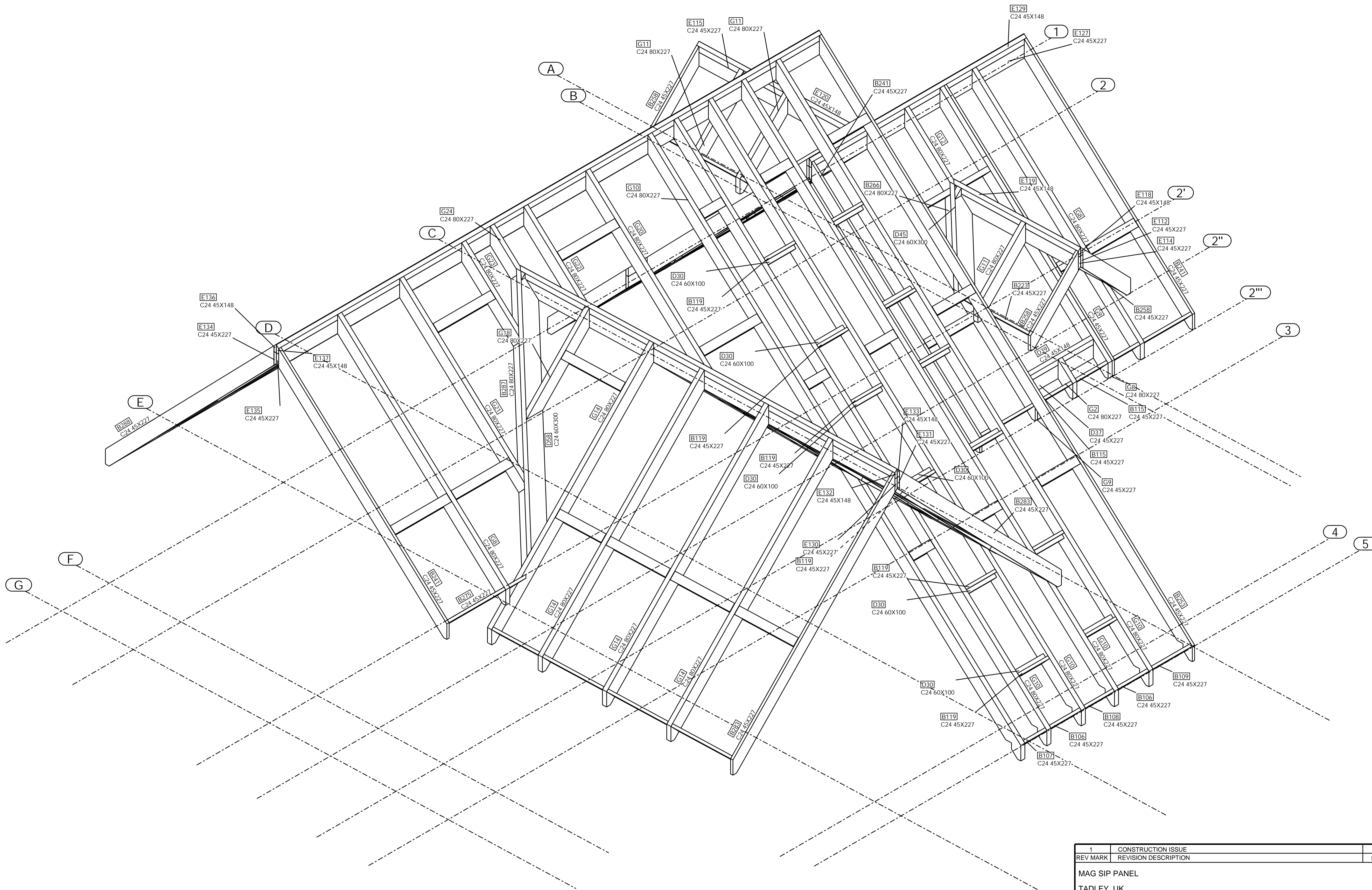
3 D ROOF VIEW (1) - EXC. MGO BOARD AND EPS
