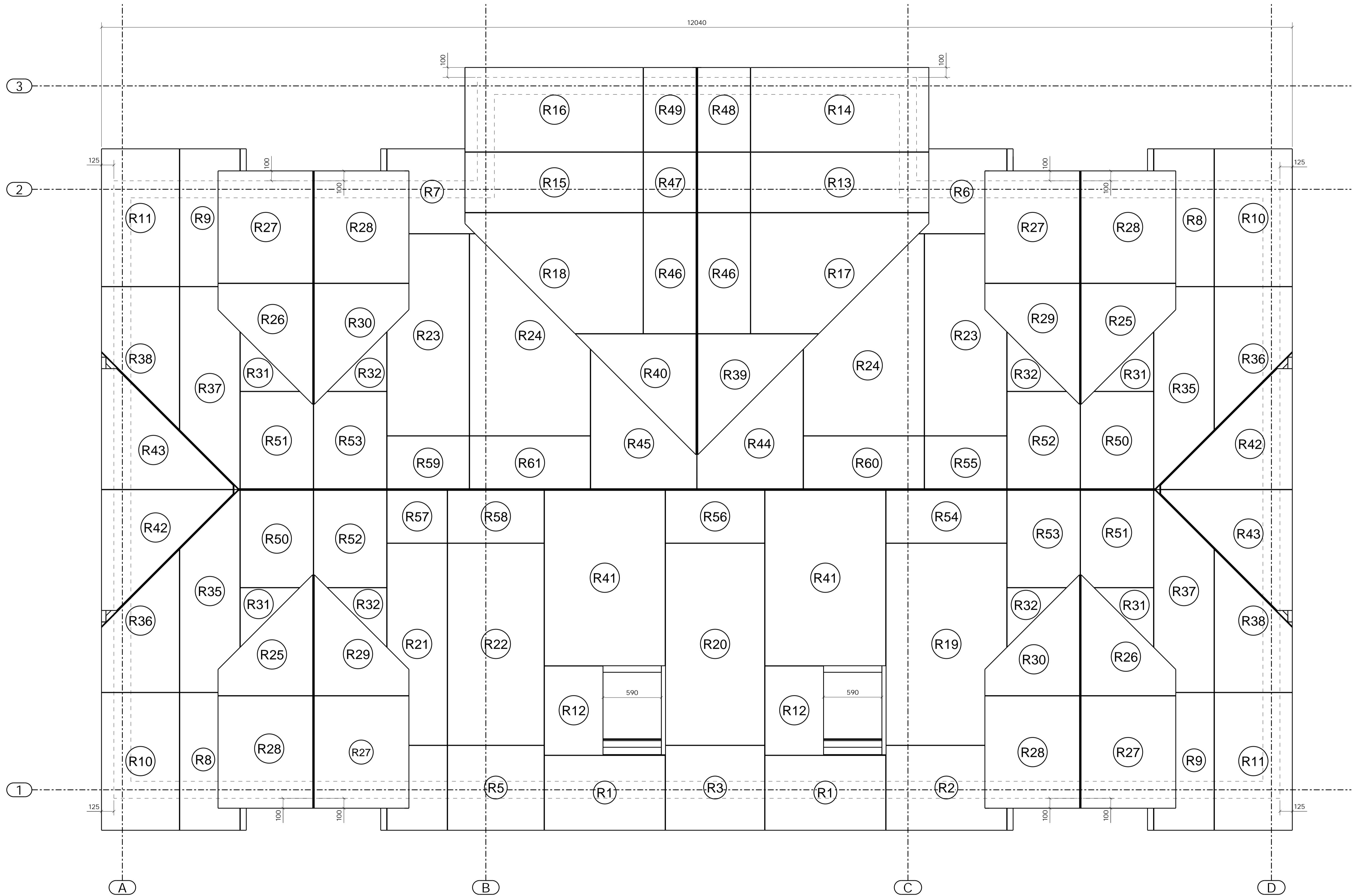
ROOF PLAN 1:20
